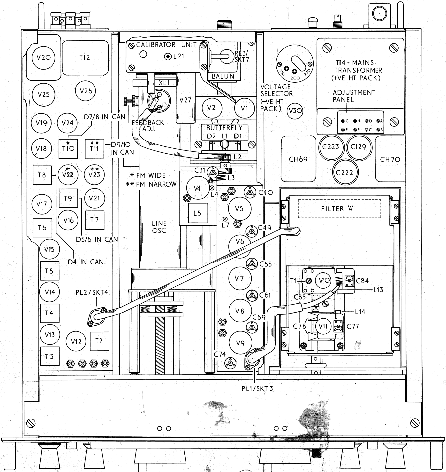
PLAN VIEW OF MODEL 770S. SHOWING MAJOR COMPONENTS AND ALIGNMENT POINTS.
